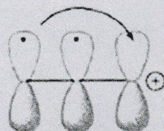
Resonance from \pi bonds
