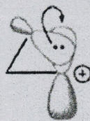
Bridging halonium ion
